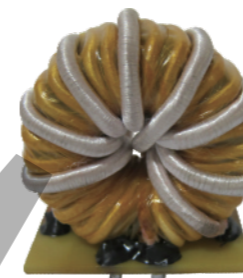
铁氧体T56X28X28 T63X38X25 T63X35X30
